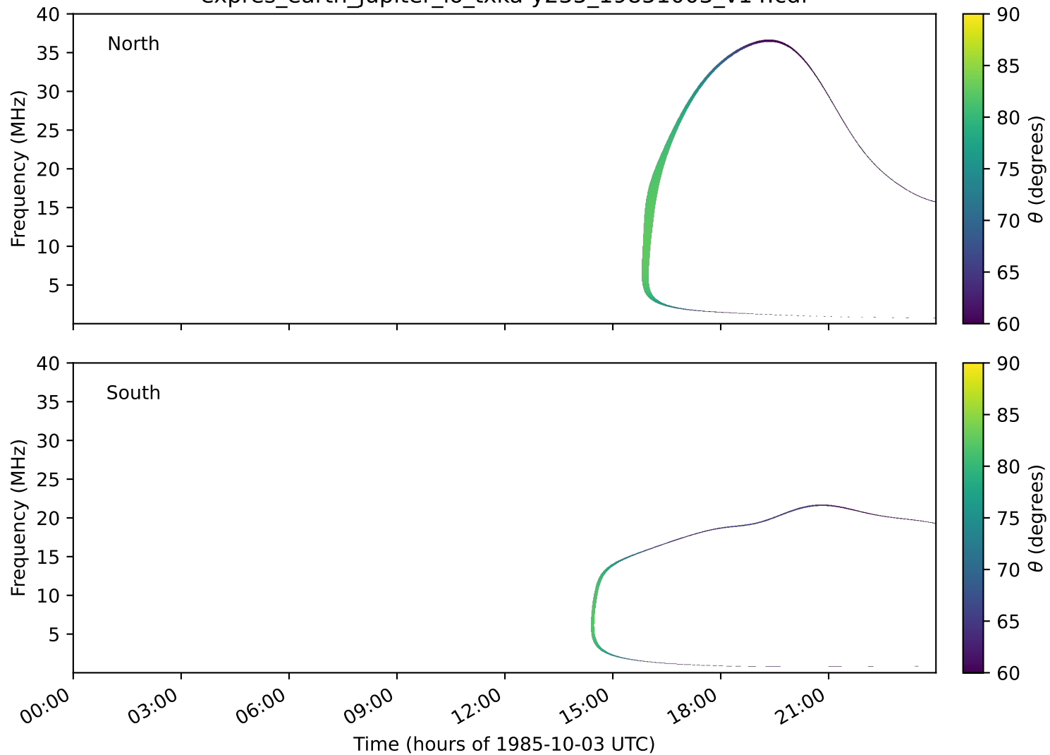
expres_earth_jupiter_io_txka-y235_19851003_v14.cdf
