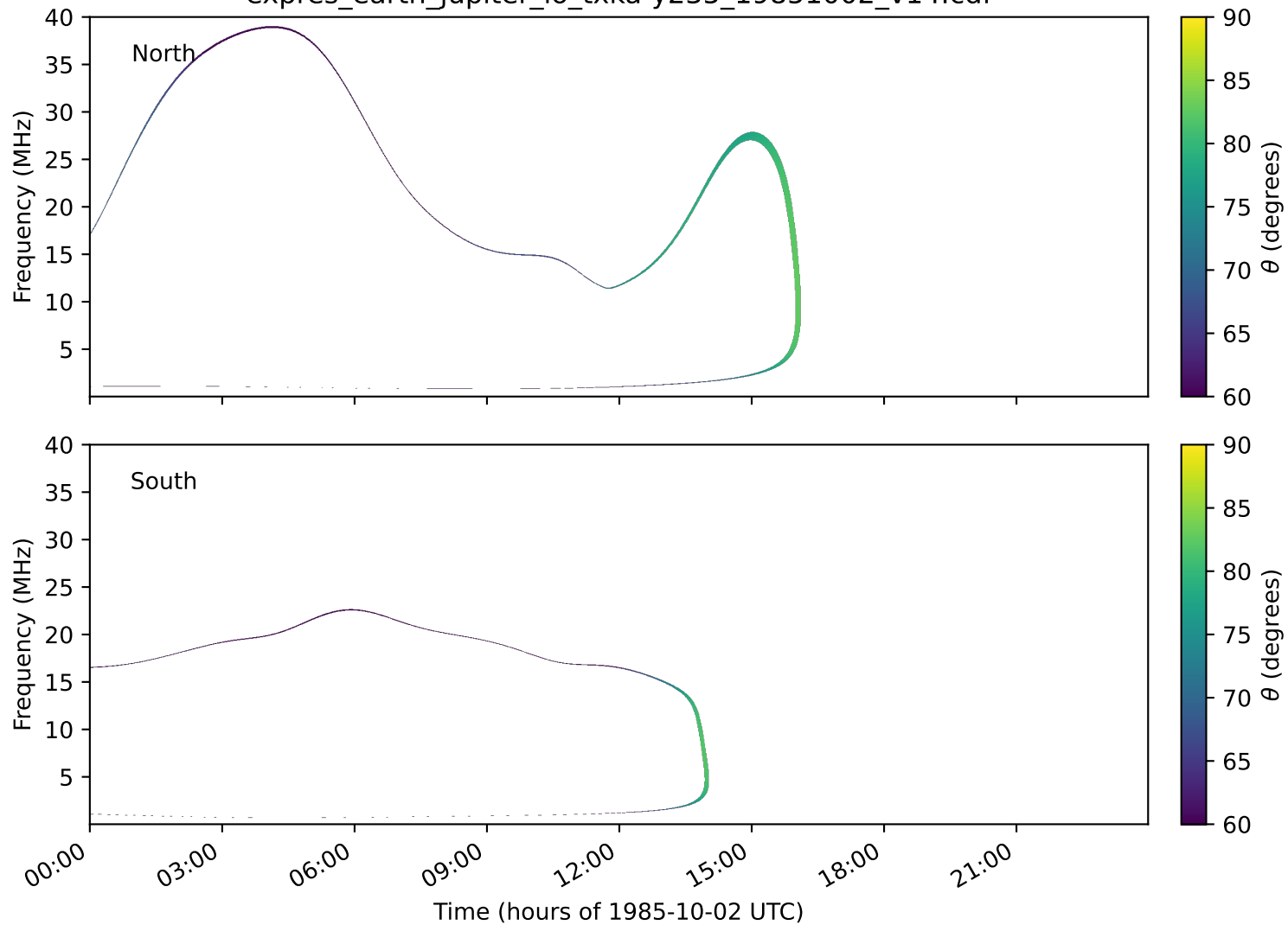
expres_earth_jupiter_io_txka-y235_19851002_v14.cdf
