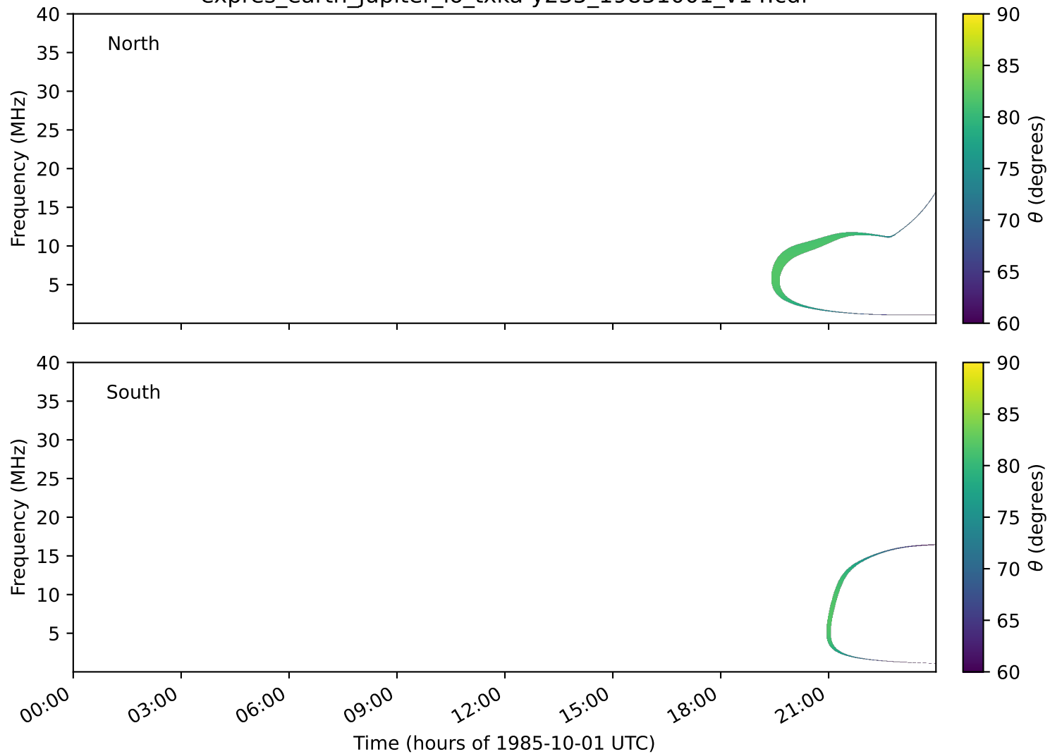
expres_earth_jupiter_io_txka-y235_19851001_v14.cdf
