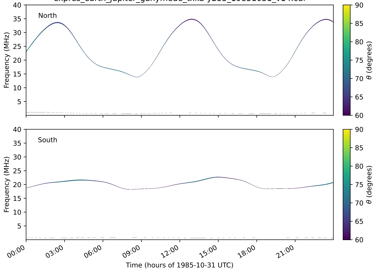
expres_earth_jupiter_ganymede_txka-y235_19851031_v14.cdf
