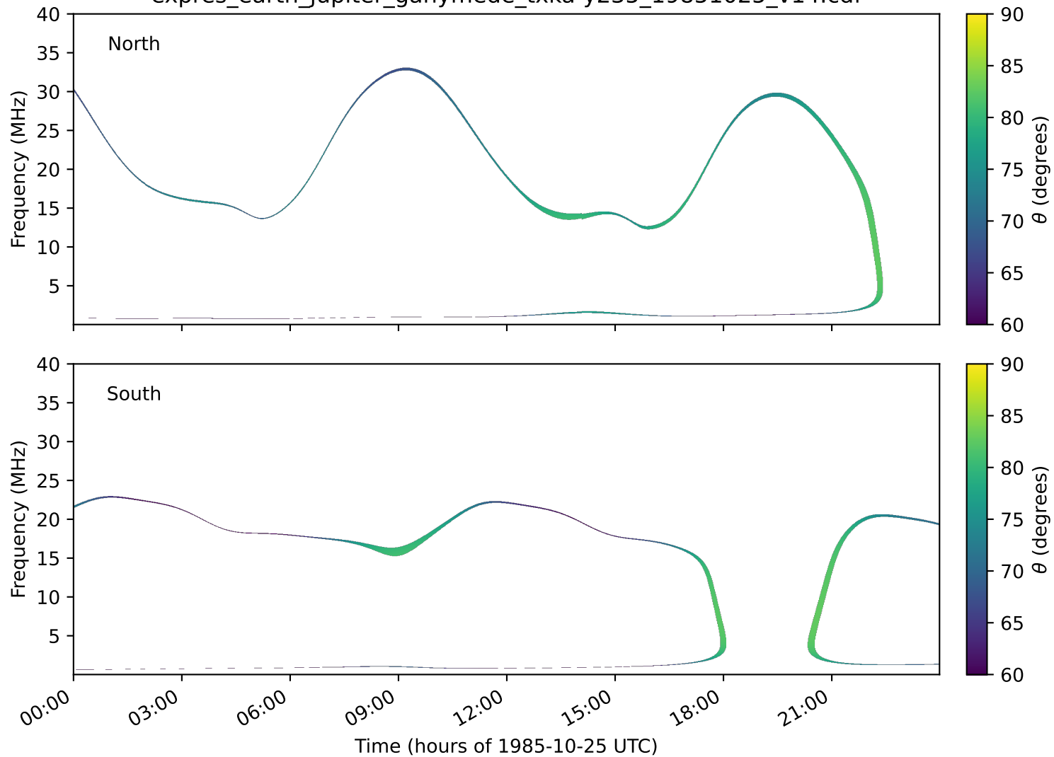
expres_earth_jupiter_ganymede_txka-y235_19851025_v14.cdf
