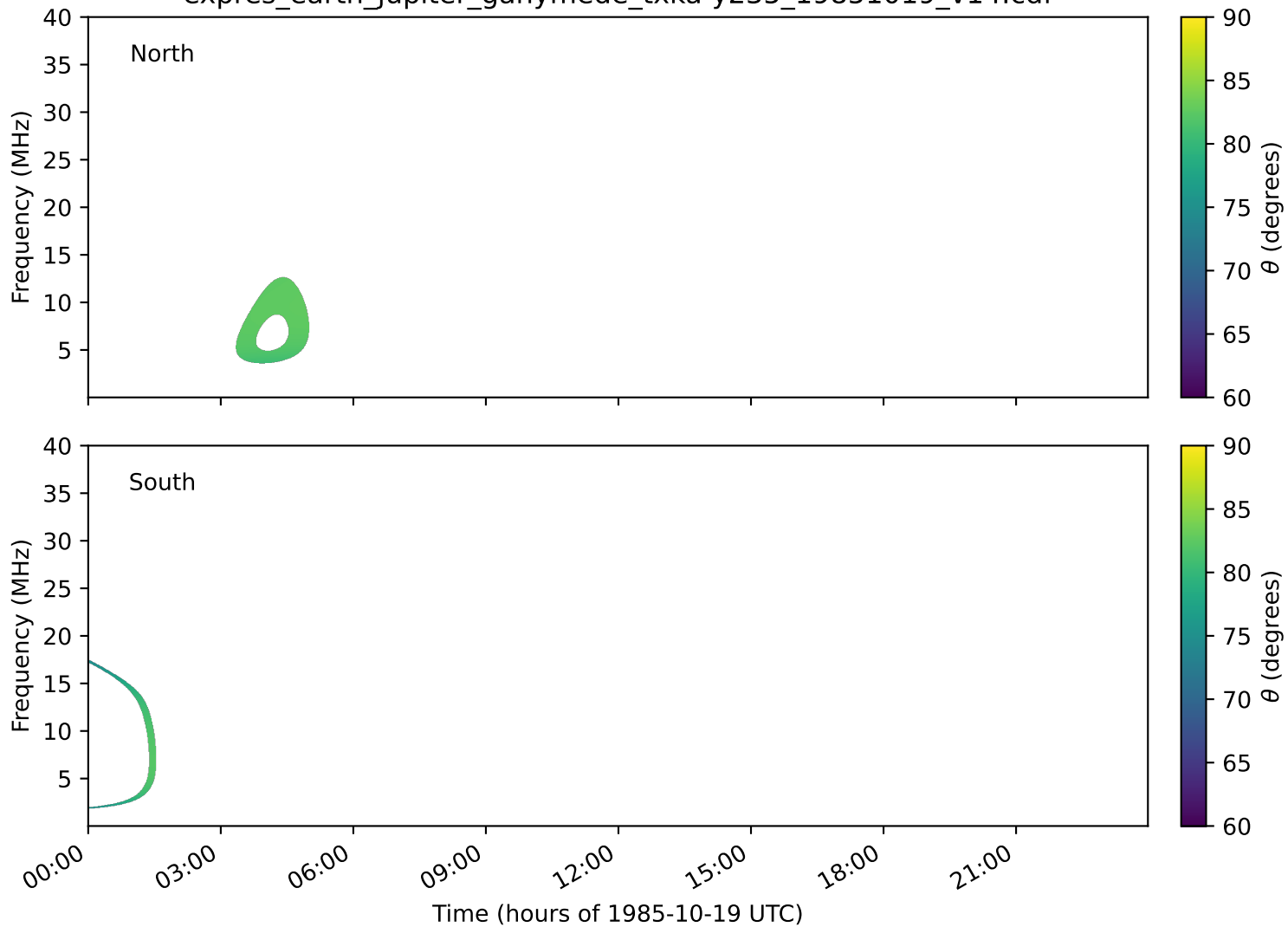
expres_earth_jupiter_ganymede_txka-y235_19851019_v14.cdf
