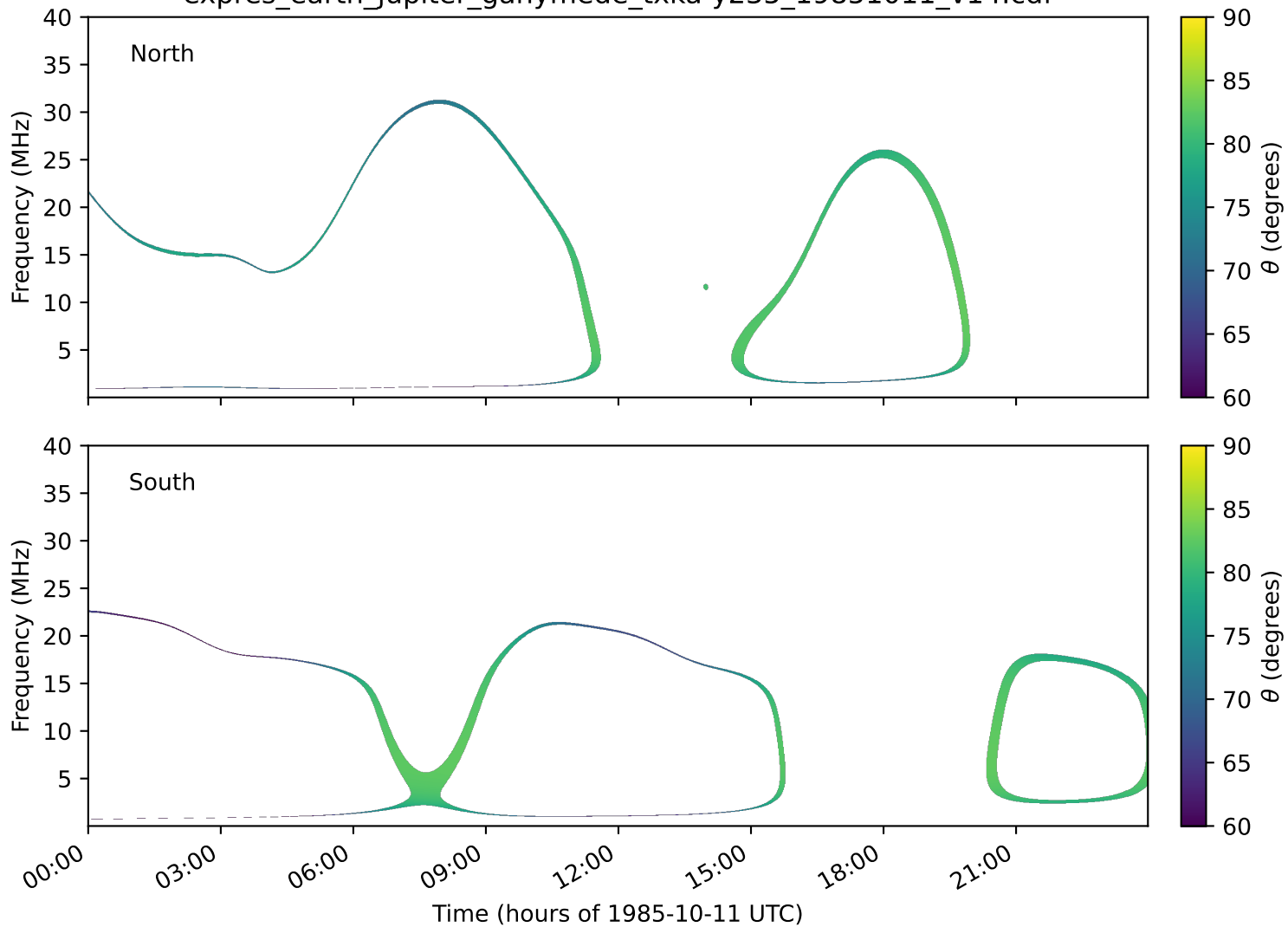
expres_earth_jupiter_ganymede_txka-y235_19851011_v14.cdf
