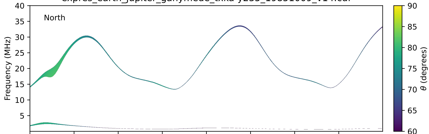
expres_earth_jupiter_ganymede_txka-y235_19851009_v14.cdf
