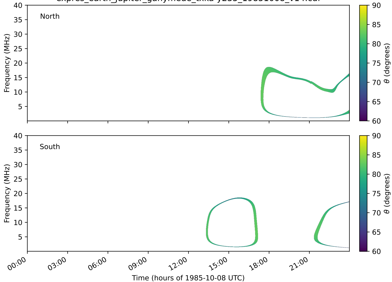
expres_earth_jupiter_ganymede_txka-y235_19851008_v14.cdf
