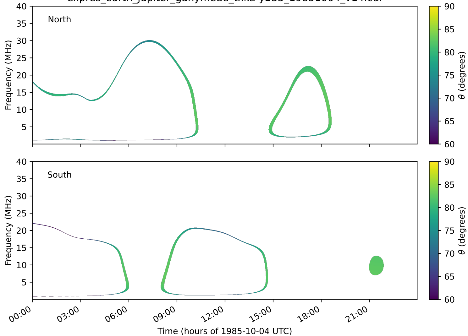
expres_earth_jupiter_ganymede_txka-y235_19851004_v14.cdf
