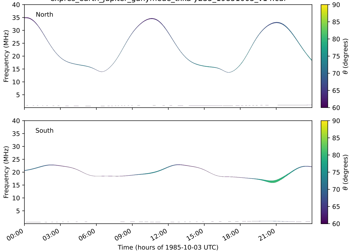
expres_earth_jupiter_ganymede_txka-y235_19851003_v14.cdf
