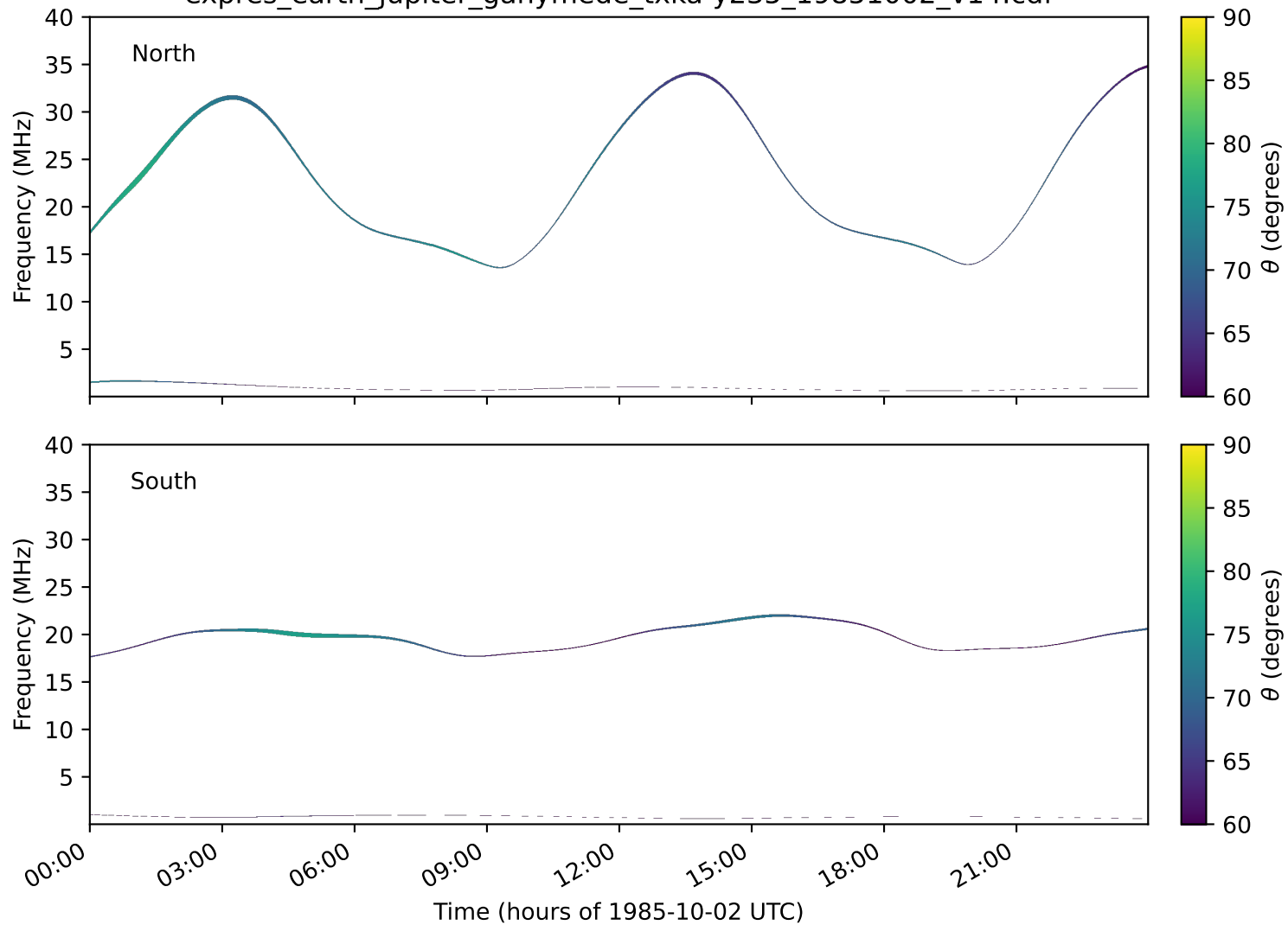
expres_earth_jupiter_ganymede_txka-y235_19851002_v14.cdf
