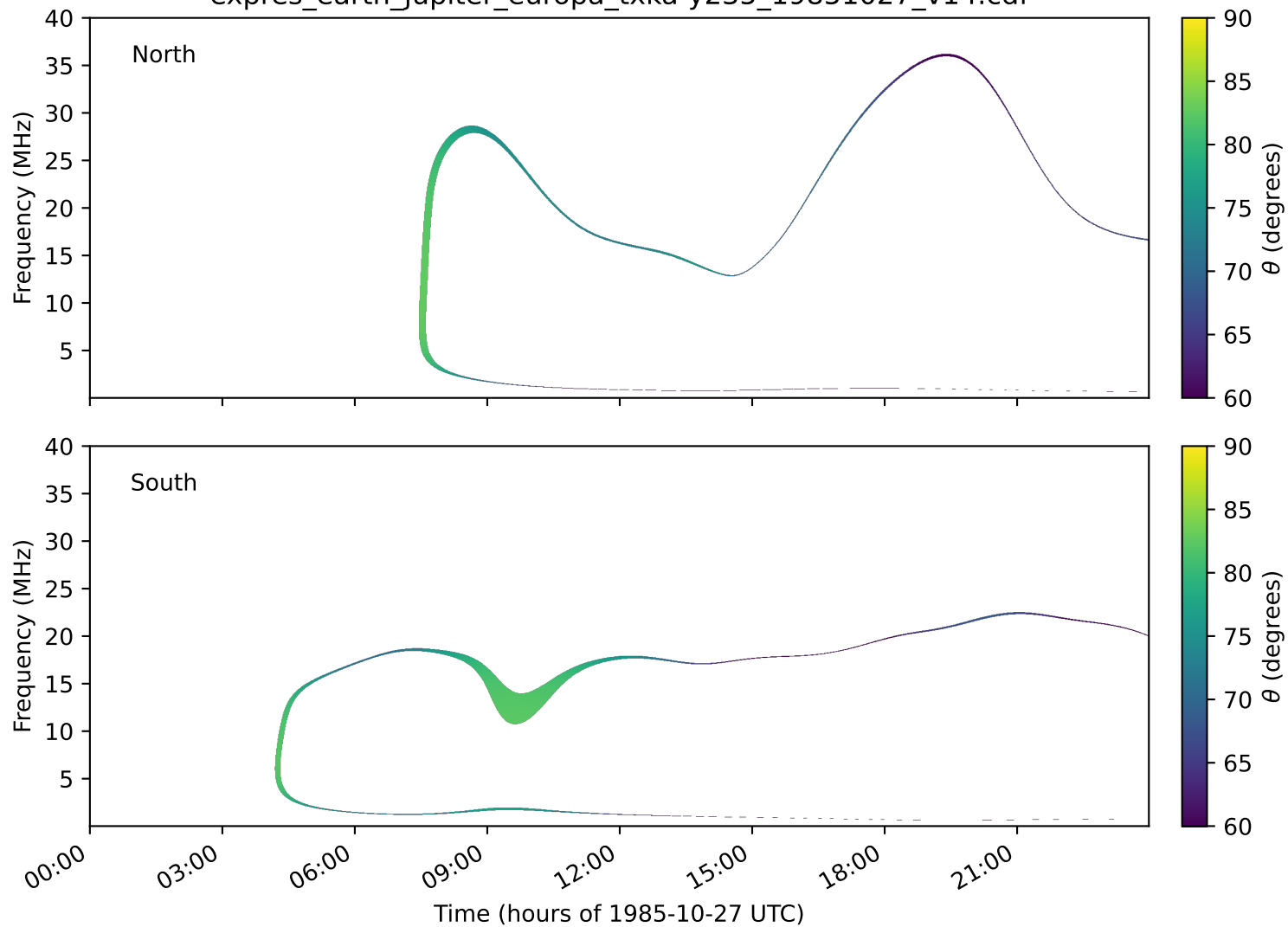
expres_earth_jupiter_europa_txka-y235_19851027_v14.cdf
