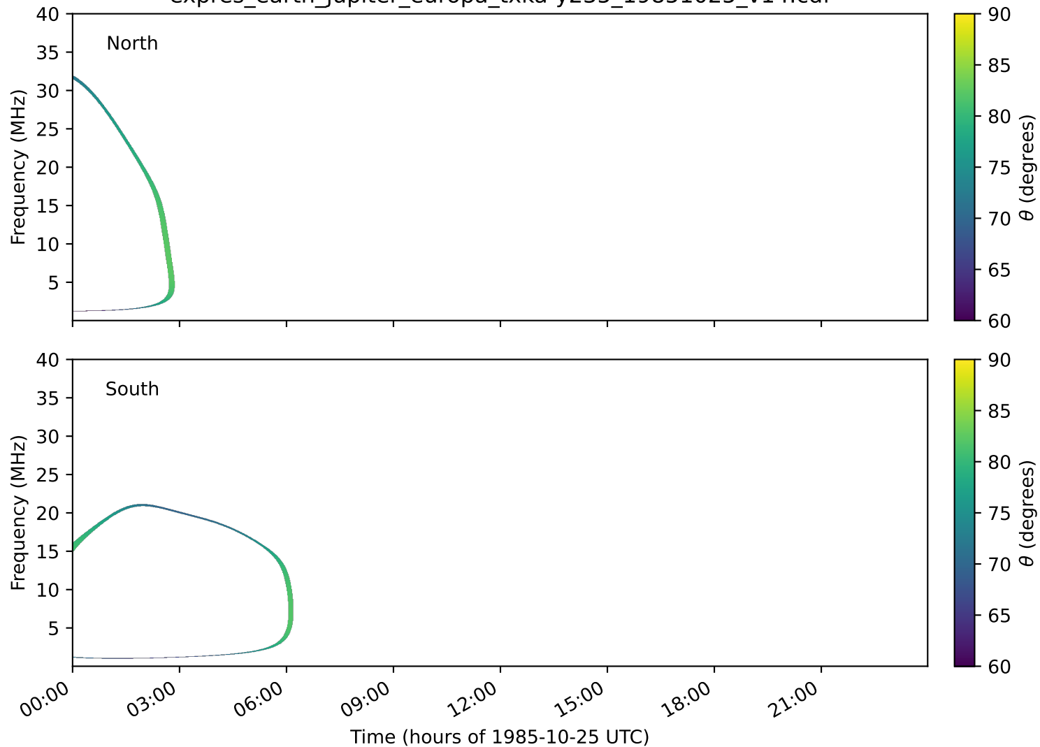
expres_earth_jupiter_europa_txka-y235_19851025_v14.cdf
