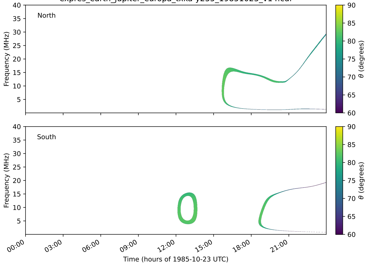
expres_earth_jupiter_europa_txka-y235_19851023_v14.cdf
