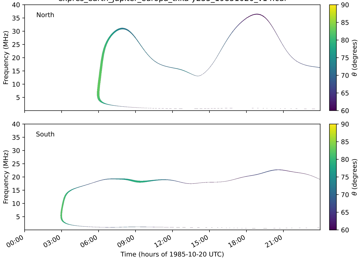
expres_earth_jupiter_europa_txka-y235_19851020_v14.cdf
