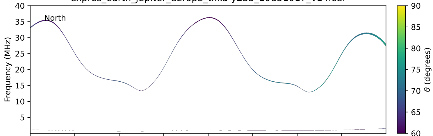
expres_earth_jupiter_europa_txka-y235_19851017_v14.cdf
