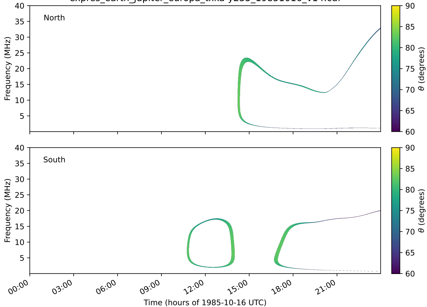
expres_earth_jupiter_europa_txka-y235_19851016_v14.cdf
