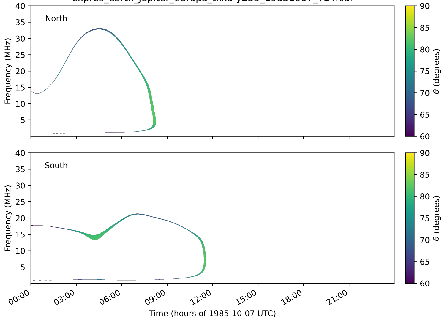
expres_earth_jupiter_europa_txka-y235_19851007_v14.cdf
