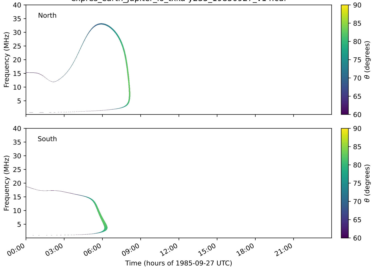
expres_earth_jupiter_io_txka-y235_19850927_v14.cdf
