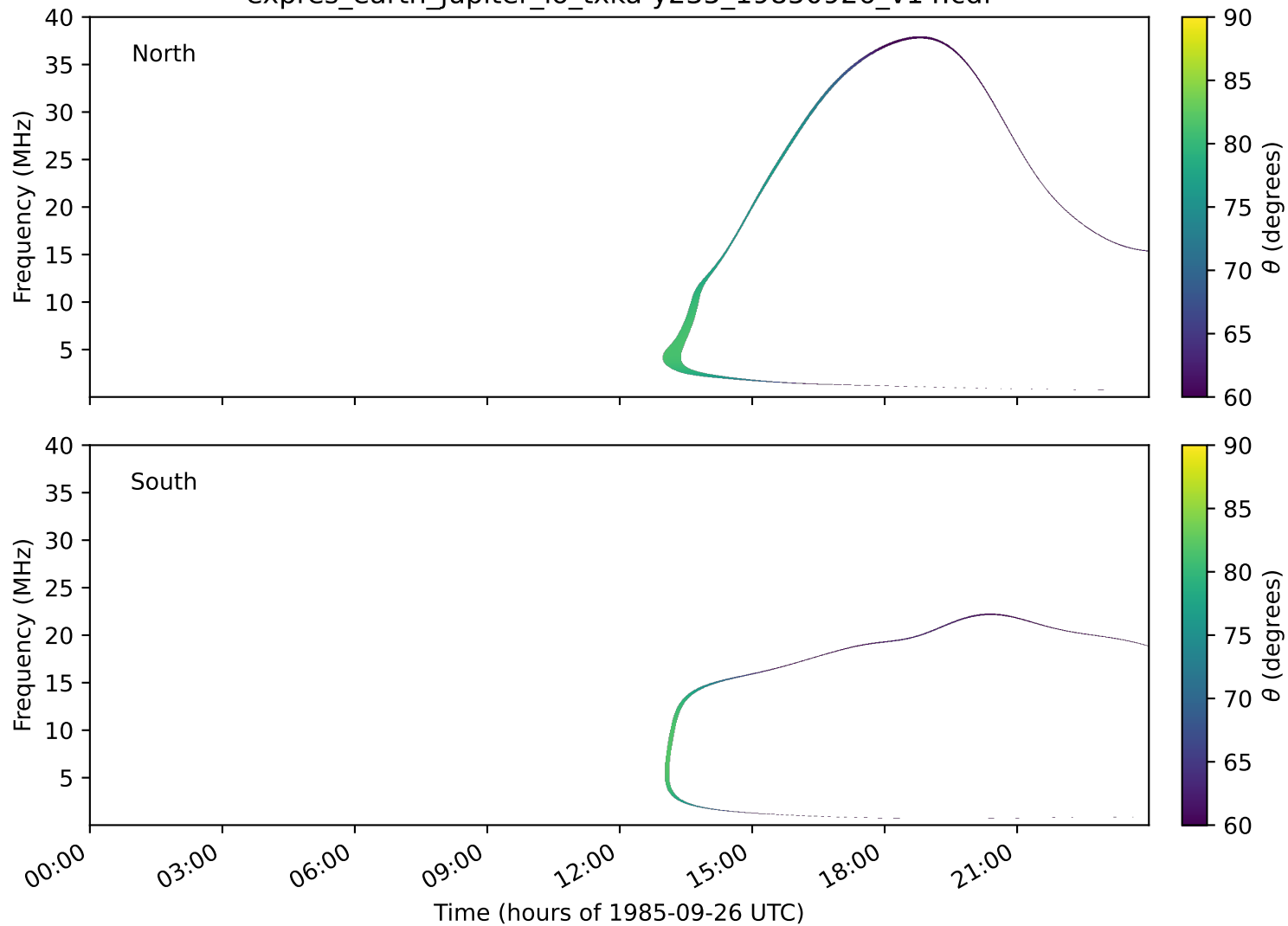
expres_earth_jupiter_io_txka-y235_19850926_v14.cdf
