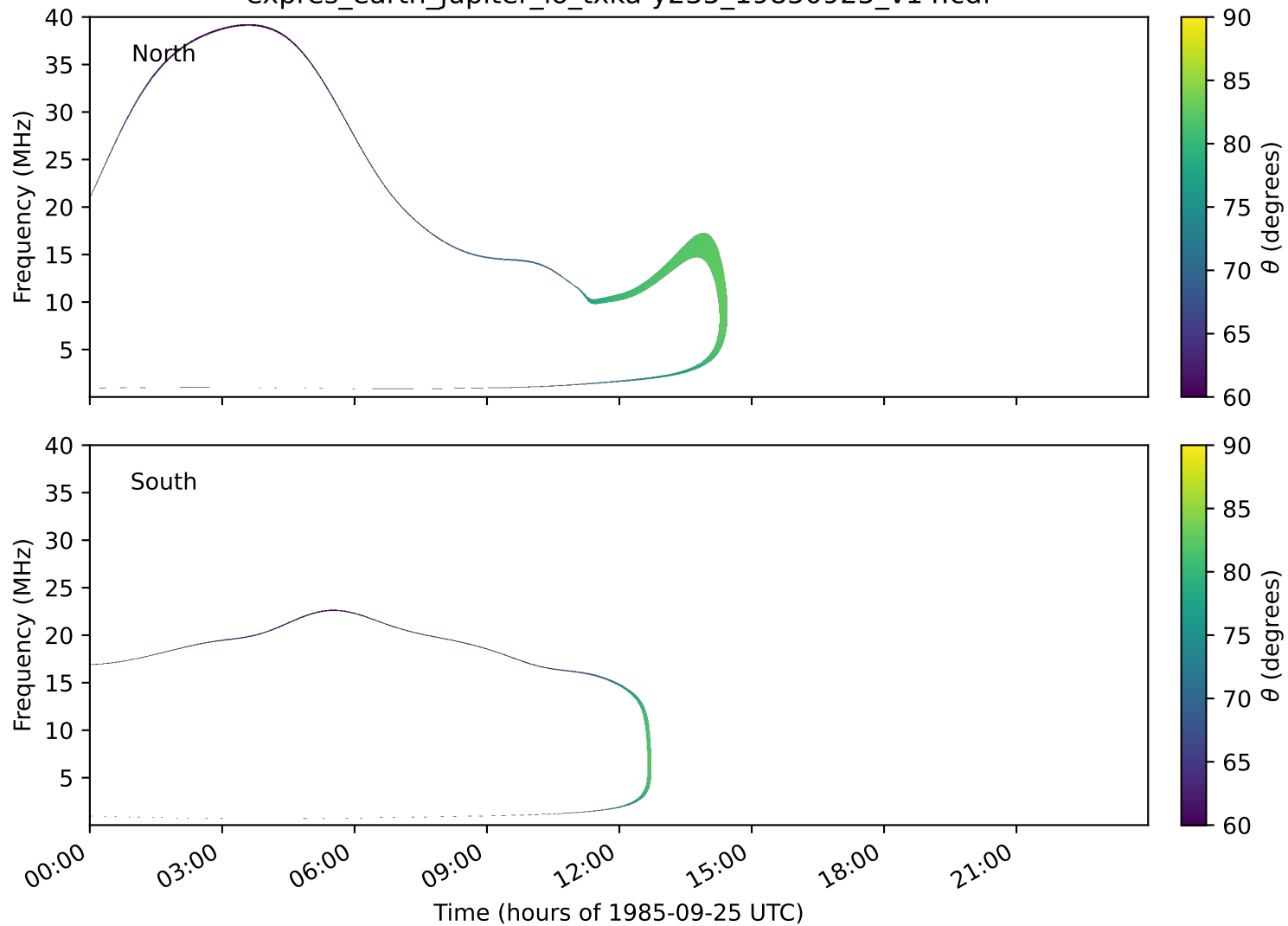
expres_earth_jupiter_io_txka-y235_19850925_v14.cdf
