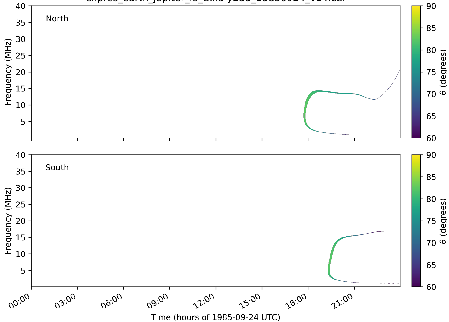
expres_earth_jupiter_io_txka-y235_19850924_v14.cdf
