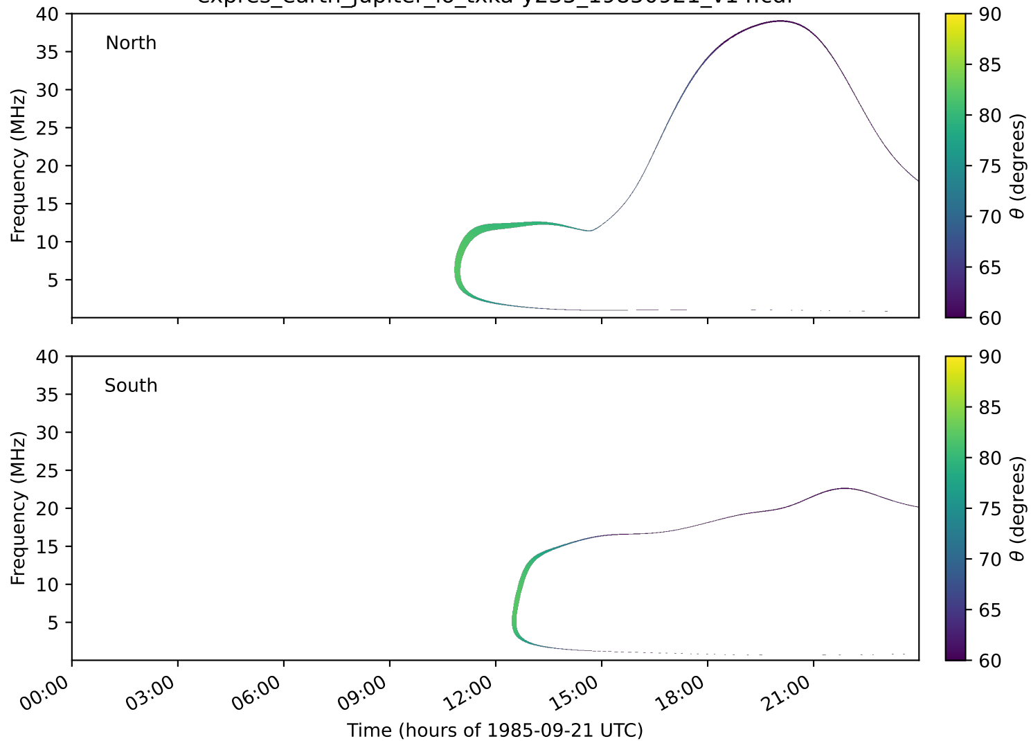
expres_earth_jupiter_io_txka-y235_19850921_v14.cdf
