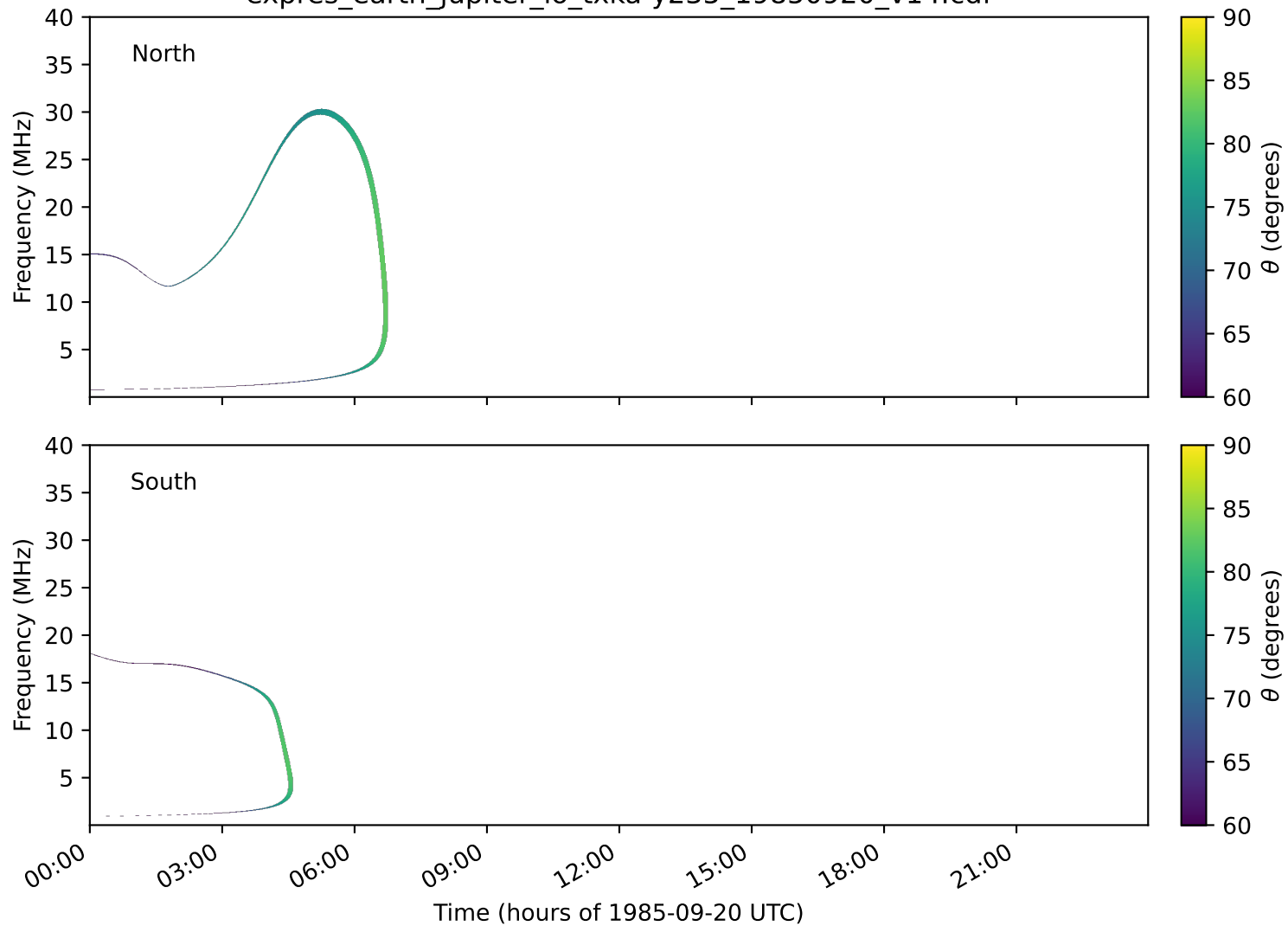
expres_earth_jupiter_io_txka-y235_19850920_v14.cdf
