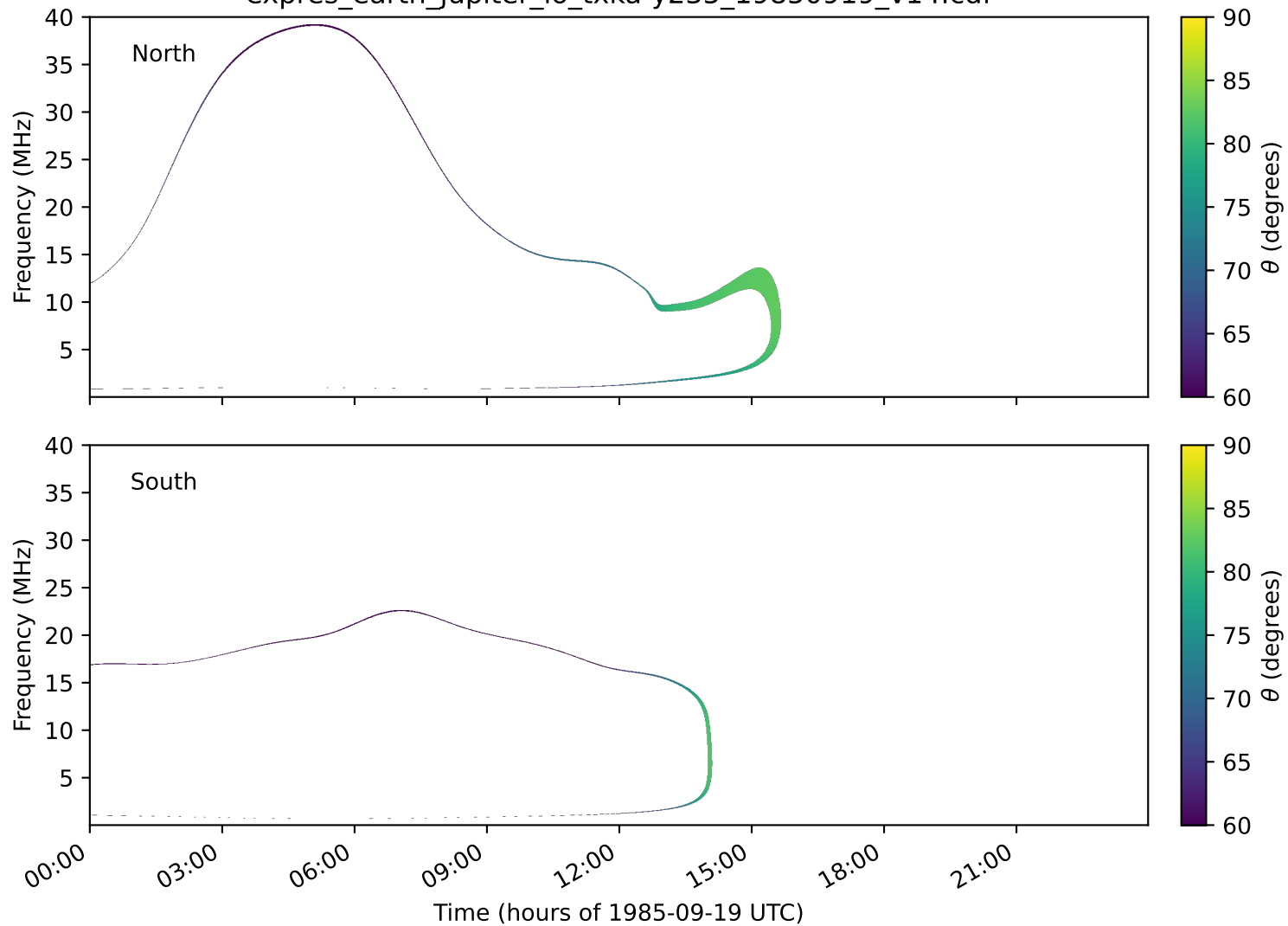
expres_earth_jupiter_io_txka-y235_19850919_v14.cdf
