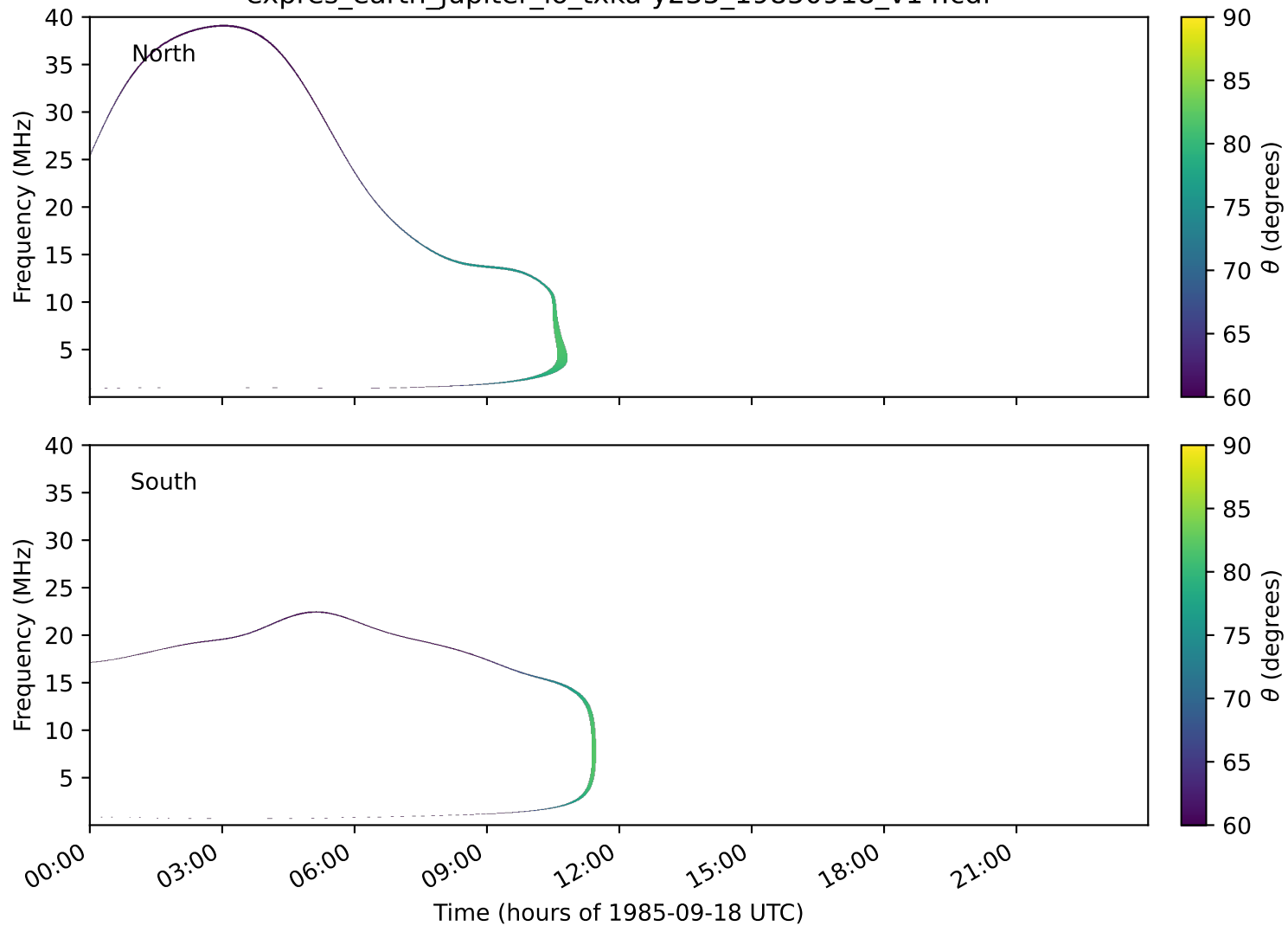
expres_earth_jupiter_io_txka-y235_19850918_v14.cdf
