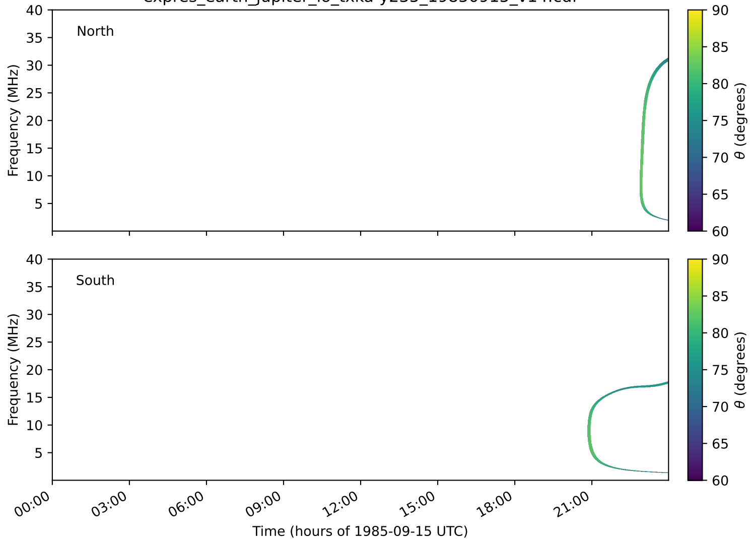
expres_earth_jupiter_io_txka-y235_19850915_v14.cdf
