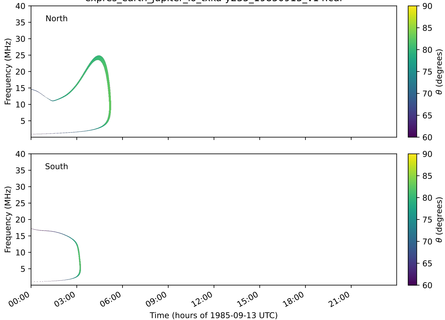
expres_earth_jupiter_io_txka-y235_19850913_v14.cdf
