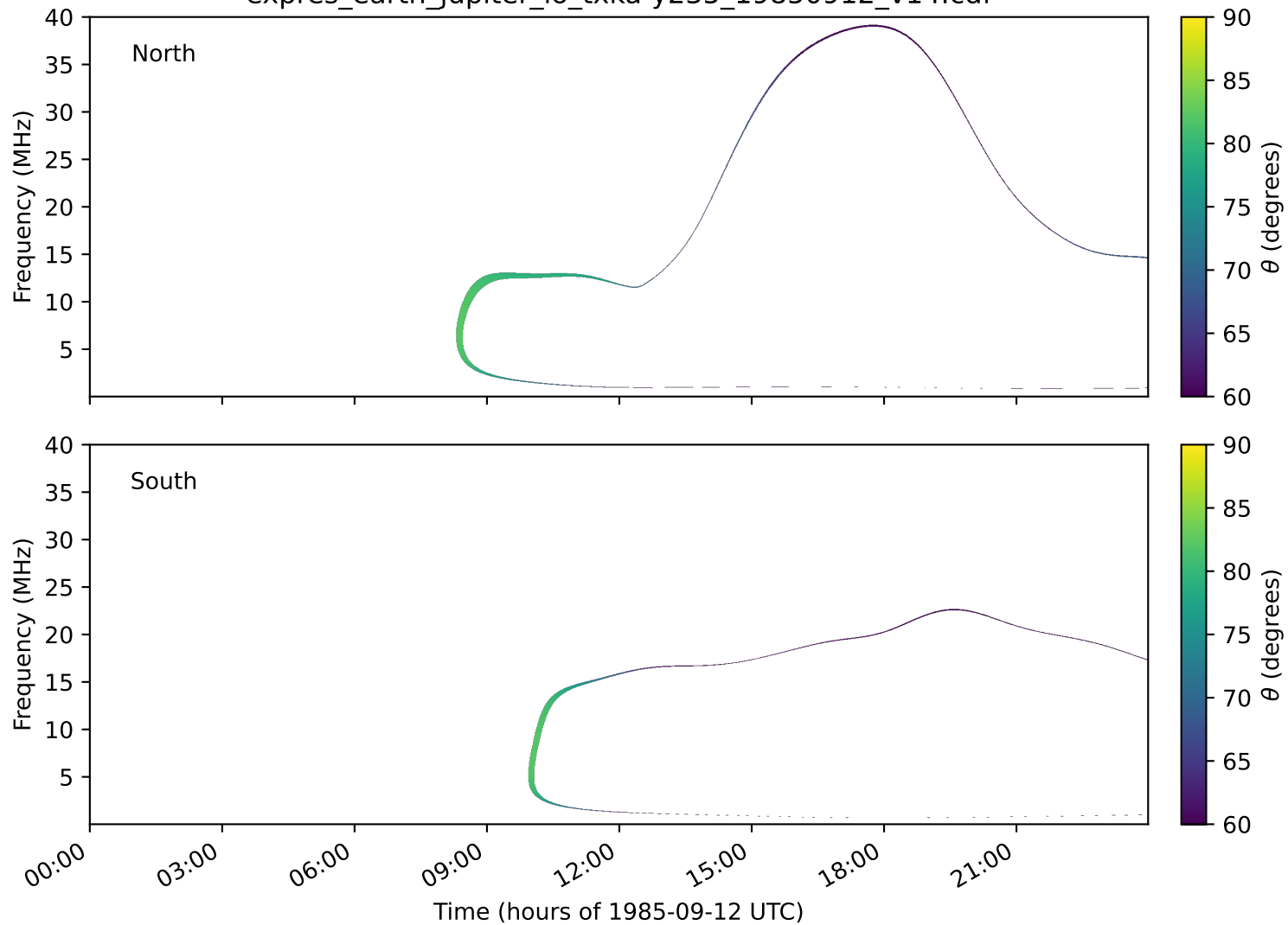
expres_earth_jupiter_io_txka-y235_19850912_v14.cdf
