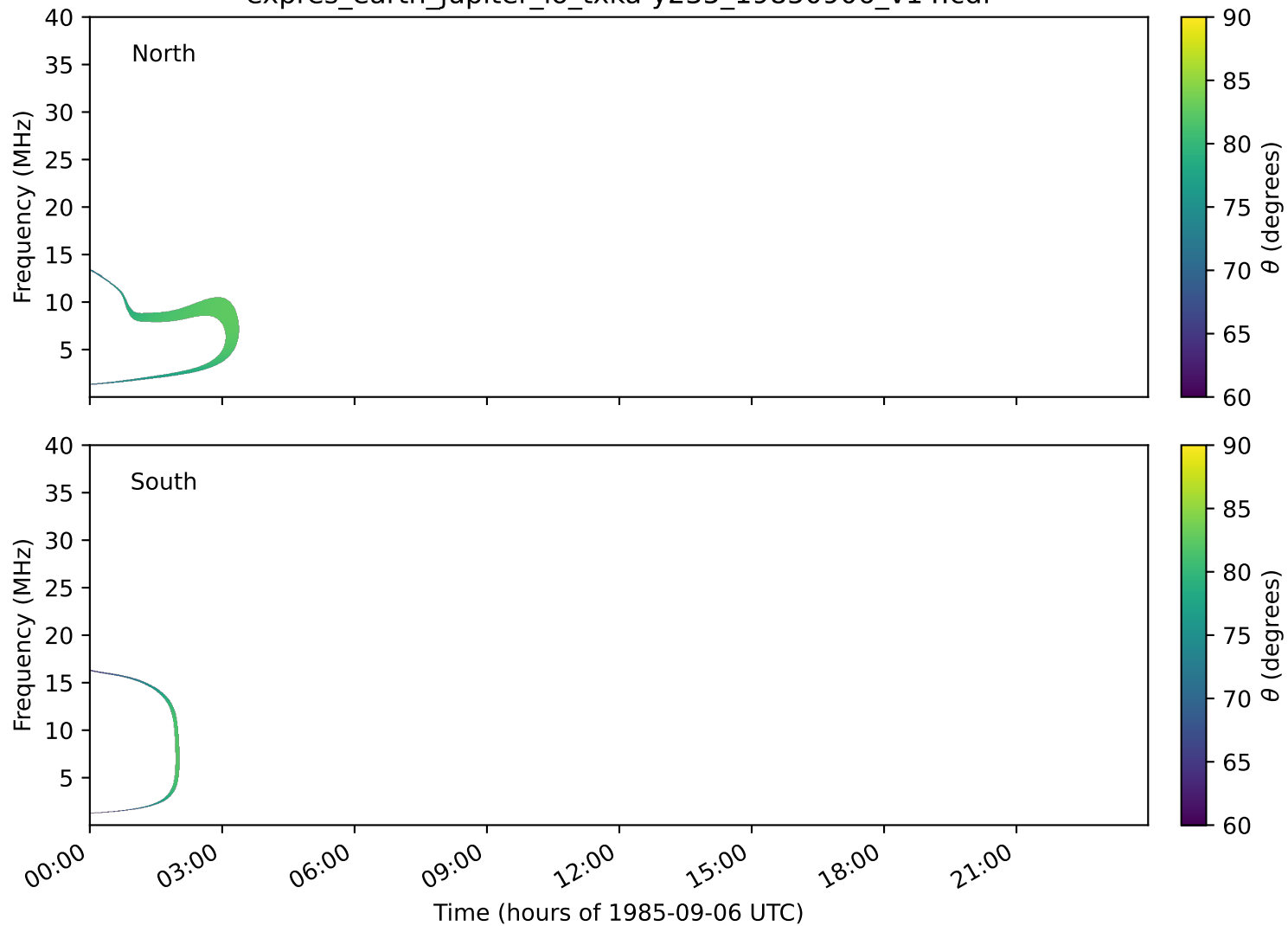
expres_earth_jupiter_io_txka-y235_19850906_v14.cdf
