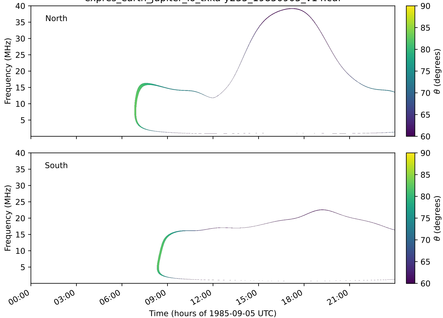
expres_earth_jupiter_io_txka-y235_19850905_v14.cdf
