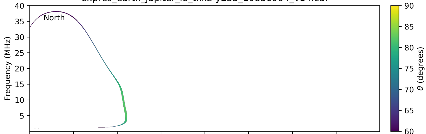
expres_earth_jupiter_io_txka-y235_19850904_v14.cdf
