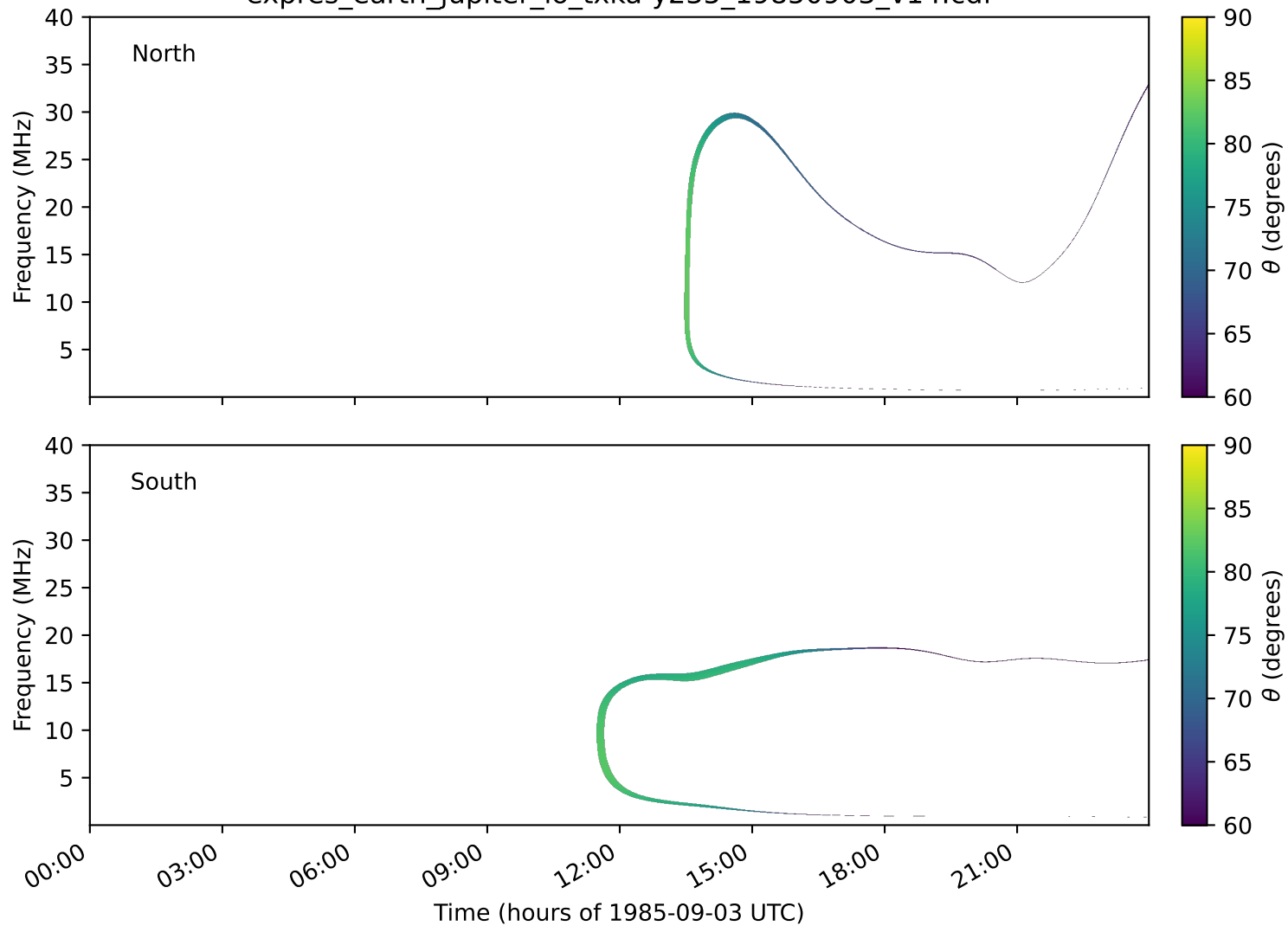
expres_earth_jupiter_io_txka-y235_19850903_v14.cdf
