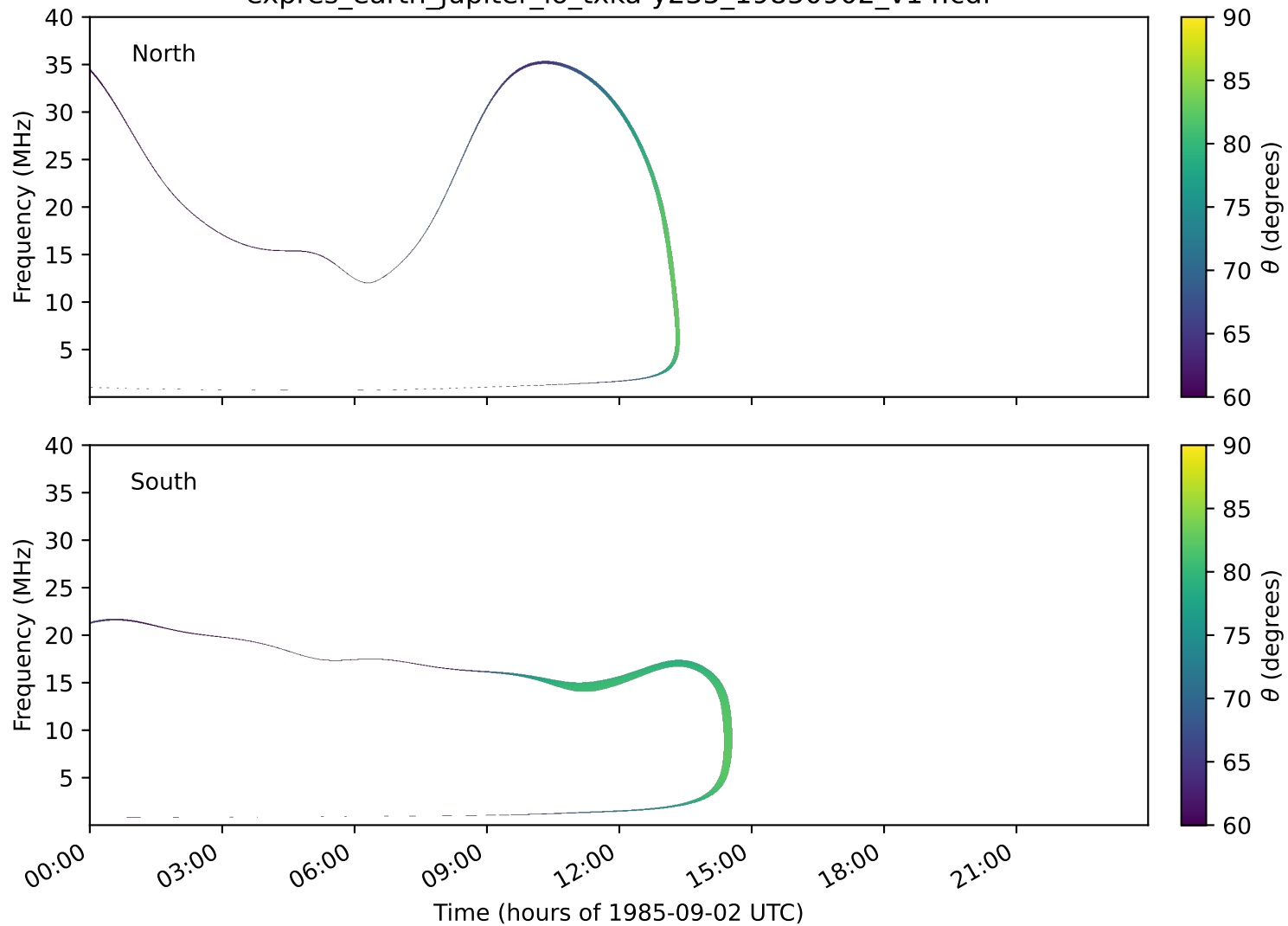
expres_earth_jupiter_io_txka-y235_19850902_v14.cdf
