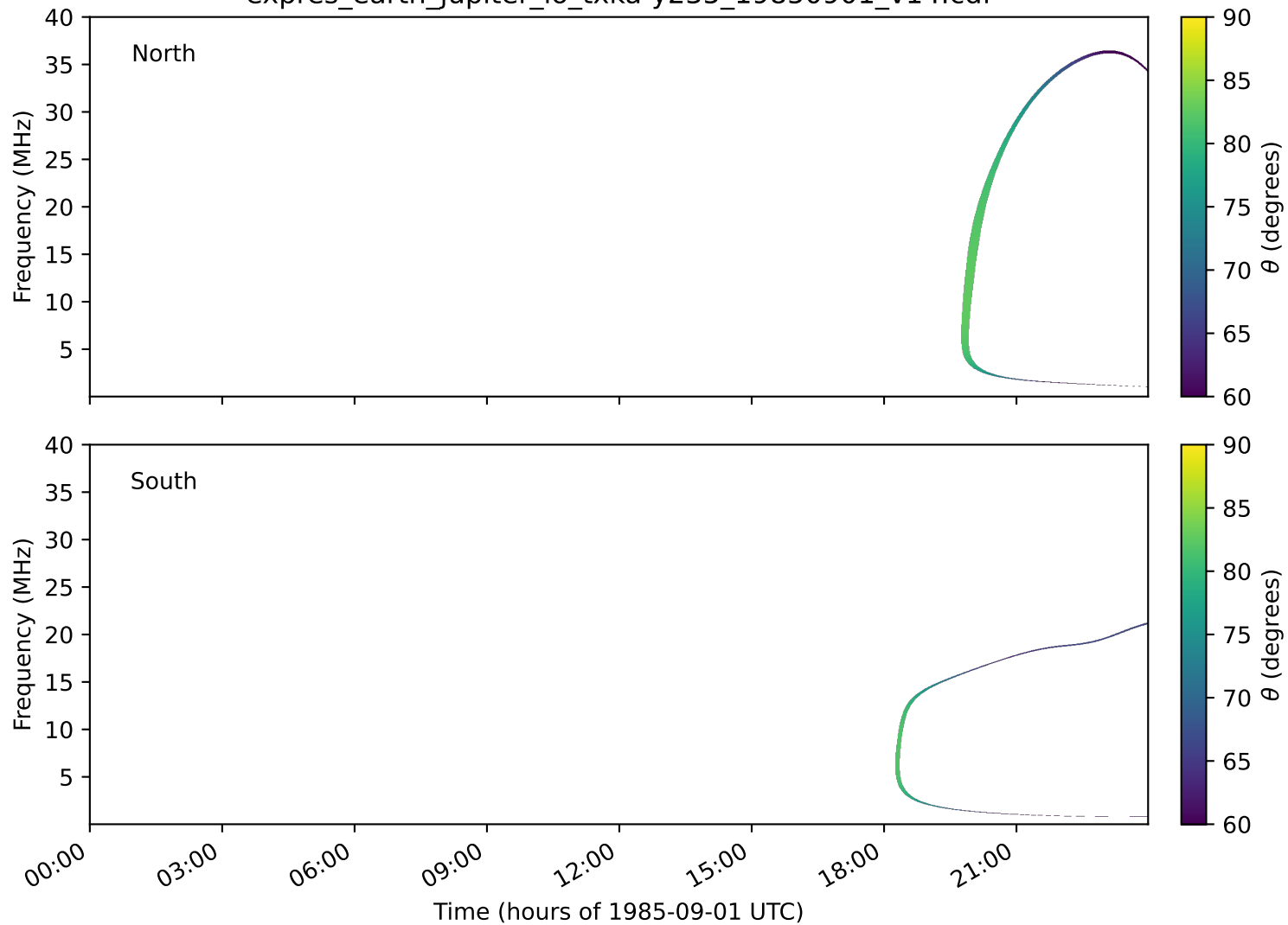
expres_earth_jupiter_io_txka-y235_19850901_v14.cdf
