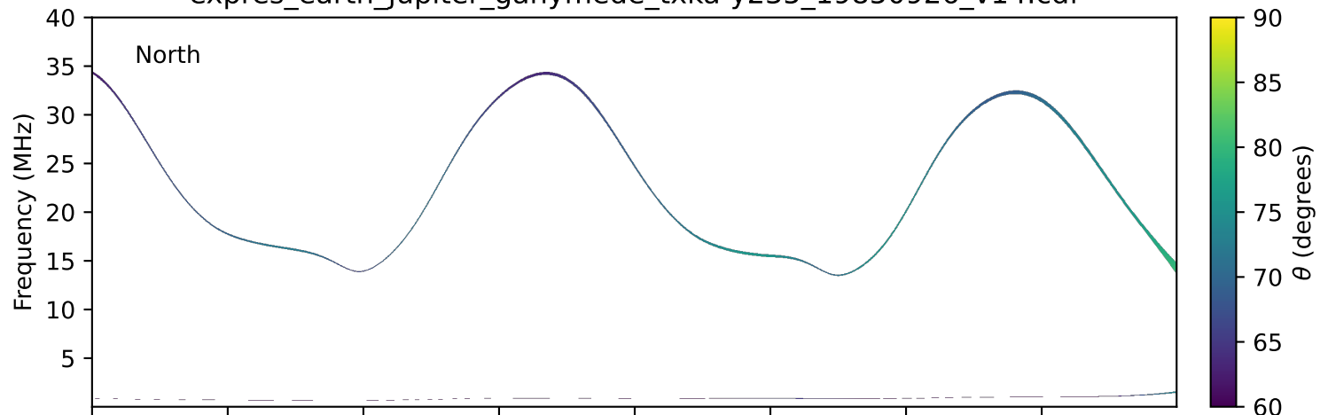
expres_earth_jupiter_ganymede_txka-y235_19850926_v14.cdf
