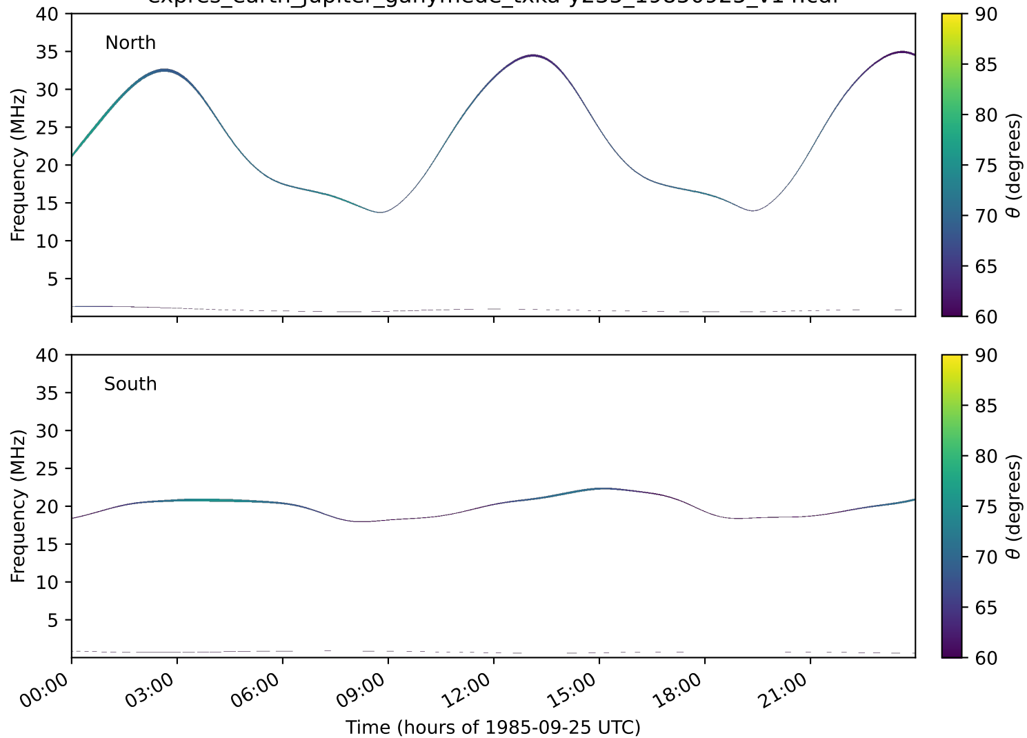
expres_earth_jupiter_ganymede_txka-y235_19850925_v14.cdf
