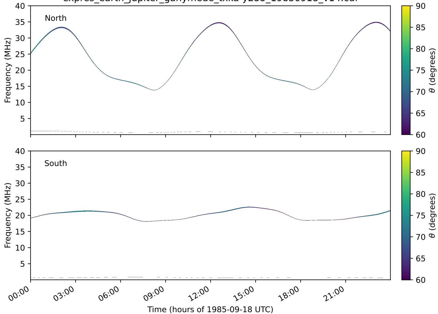
expres_earth_jupiter_ganymede_txka-y235_19850918_v14.cdf
