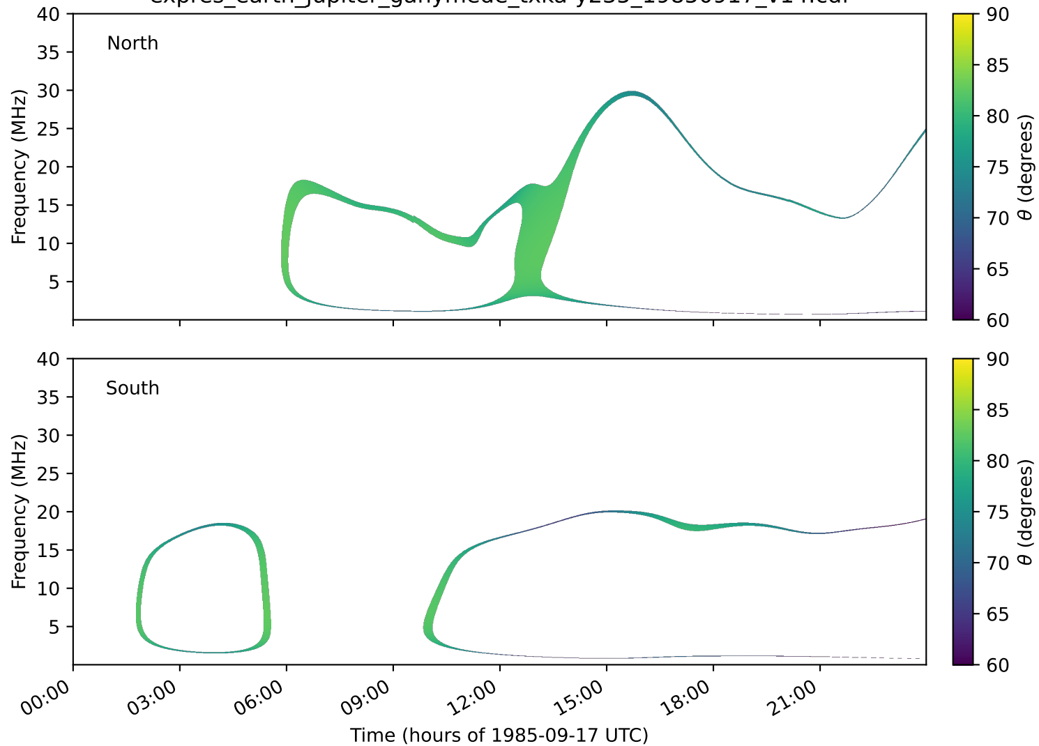
expres_earth_jupiter_ganymede_txka-y235_19850917_v14.cdf
