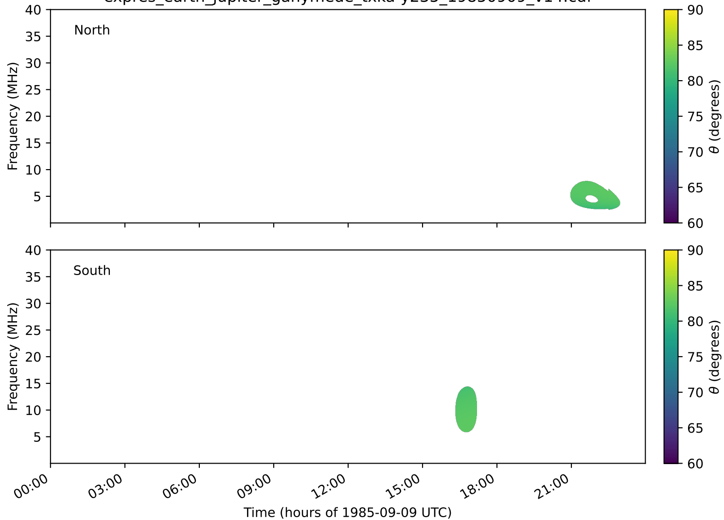
expres_earth_jupiter_ganymede_txka-y235_19850909_v14.cdf
