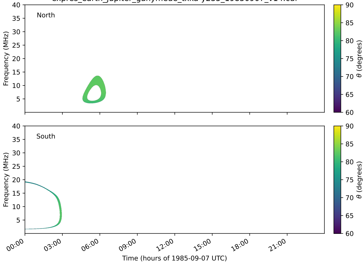
expres_earth_jupiter_ganymede_txka-y235_19850907_v14.cdf
