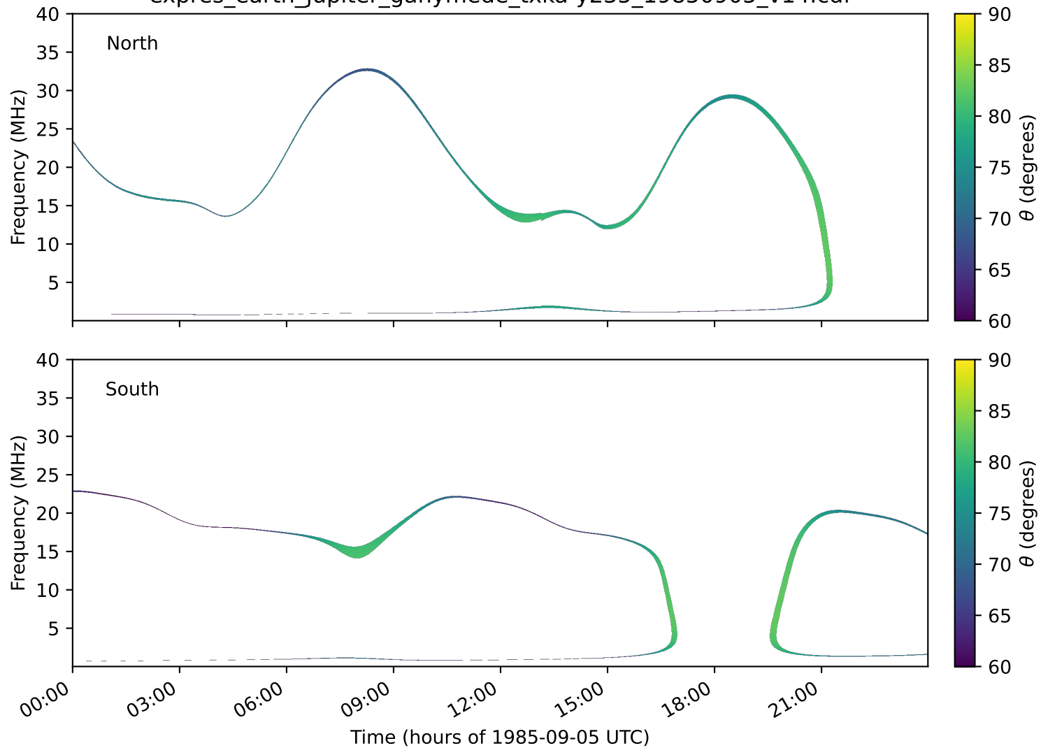
expres_earth_jupiter_ganymede_txka-y235_19850905_v14.cdf
