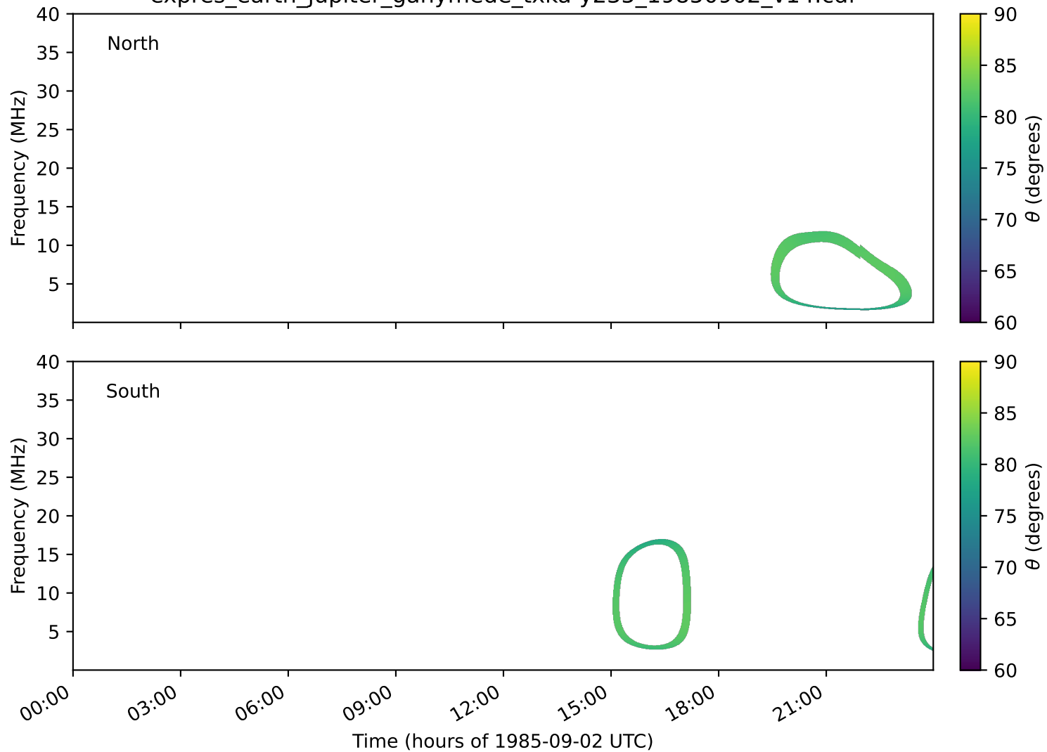
expres_earth_jupiter_ganymede_txka-y235_19850902_v14.cdf
