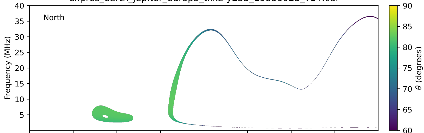
expres_earth_jupiter_europa_txka-y235_19850925_v14.cdf
