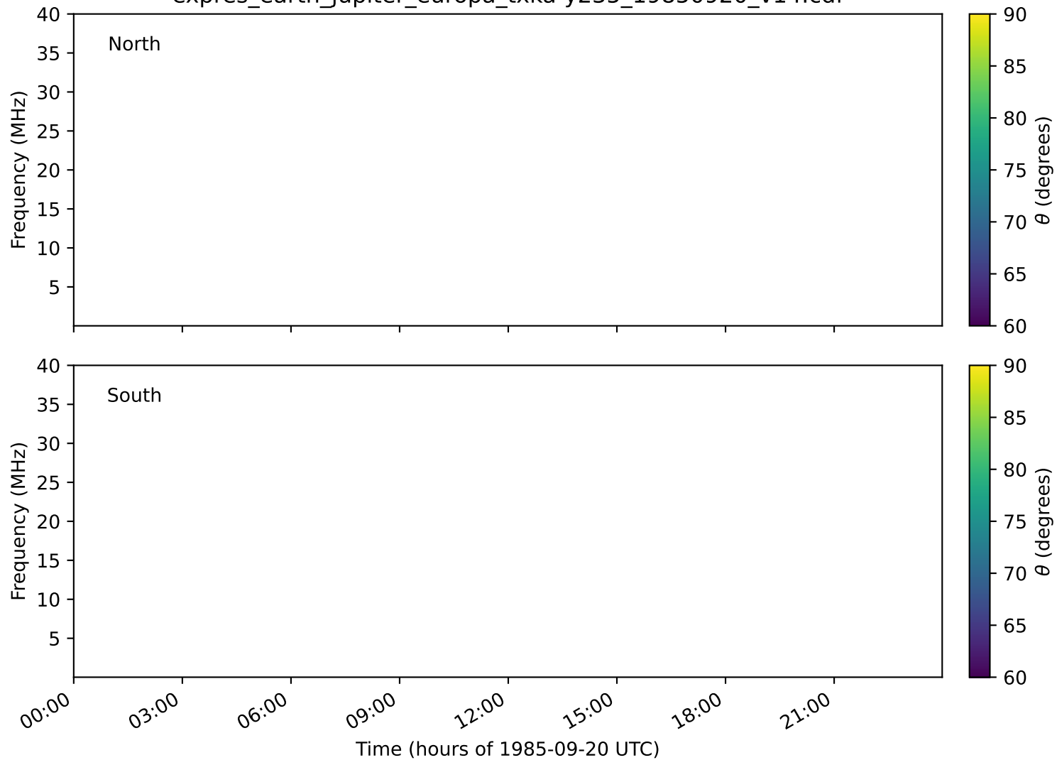
expres_earth_jupiter_europa_txka-y235_19850920_v14.cdf
