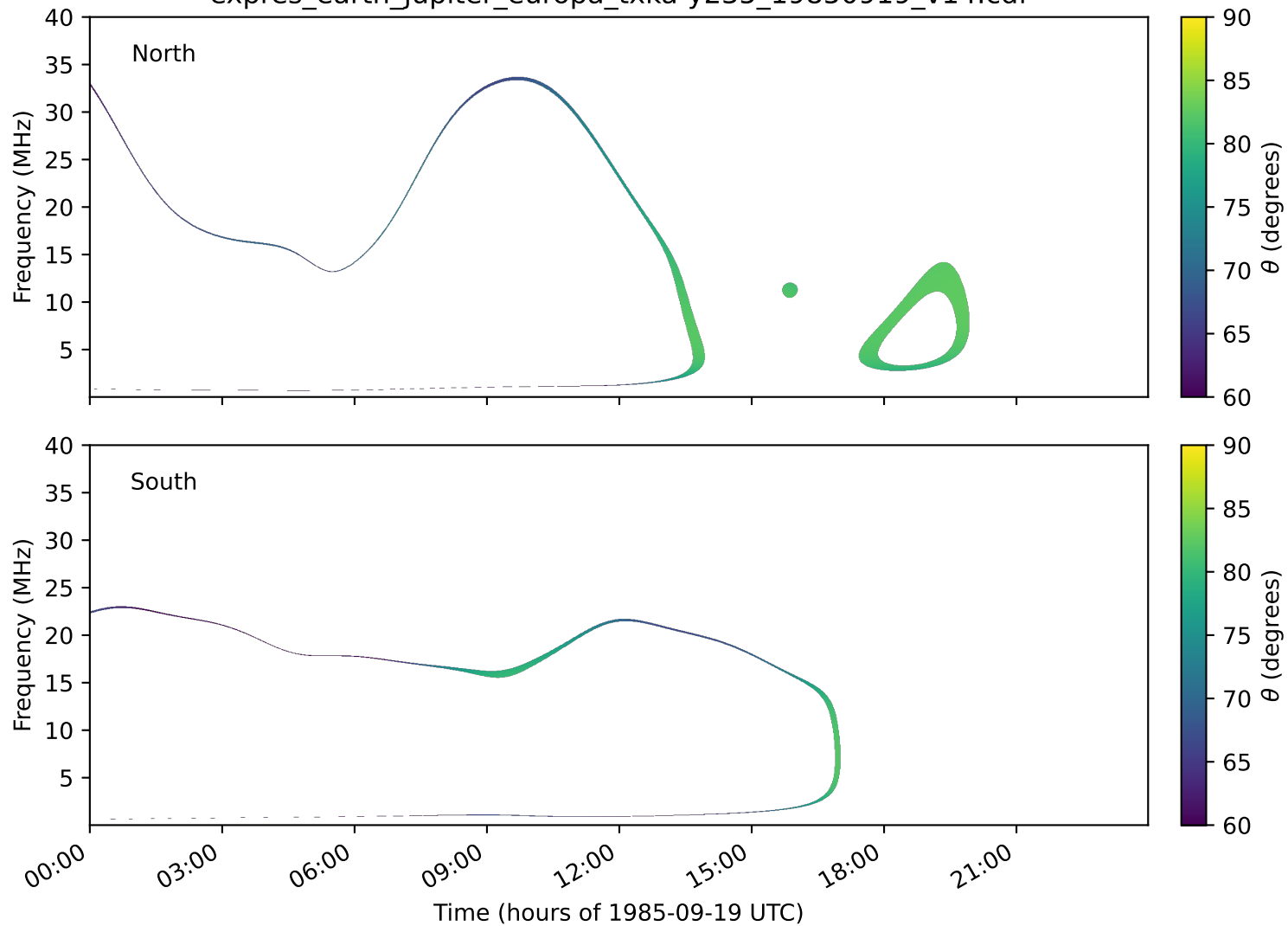
expres_earth_jupiter_europa_txka-y235_19850919_v14.cdf
