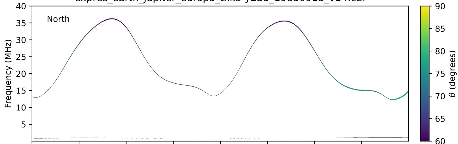
expres_earth_jupiter_europa_txka-y235_19850915_v14.cdf
