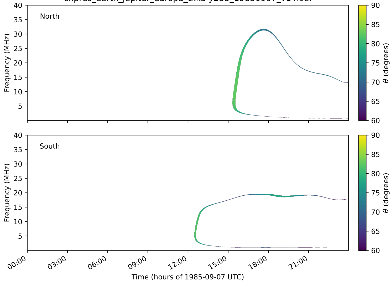
expres_earth_jupiter_europa_txka-y235_19850907_v14.cdf
