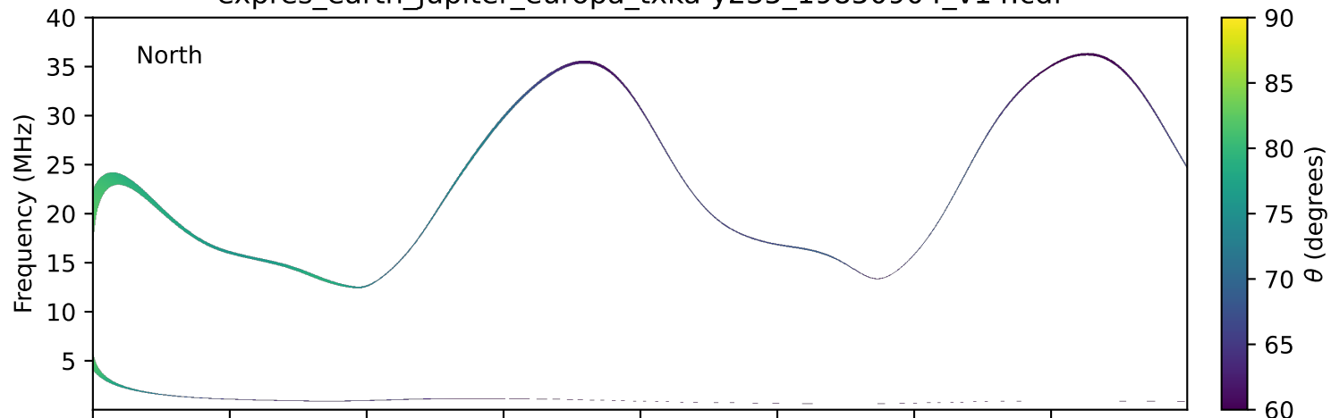
expres_earth_jupiter_europa_txka-y235_19850904_v14.cdf
